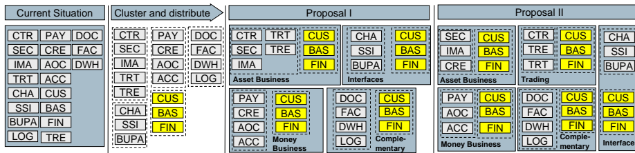
Fig. 1. Domains and their distribution in the proposals limiting failure propagation
