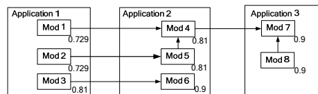
Fig. 3. Calculating failureProbability on information according to Figure 2
